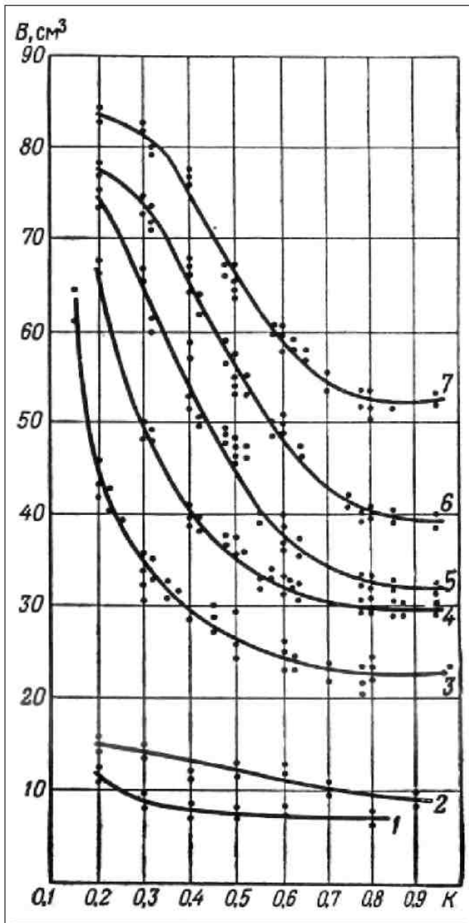
Figure 3. Dependence of filtration of VLR-stabilized drilling mud, on rate of clay colloid characteristics ( K ) [4]: 1/2-filtration in normal conditions of solutions with density 1,4 and 2,0 \text{g}/\text{cm}^3 ; 3-filtration at T = 140^\circ\text{C} and P = 5 Mpa of unweighed solution; 4-7-filtration of solutions with density 1,4; 1,6; 1,8; 2,0 \text{g}/\text{cm}^3 respectively in similar conditions
